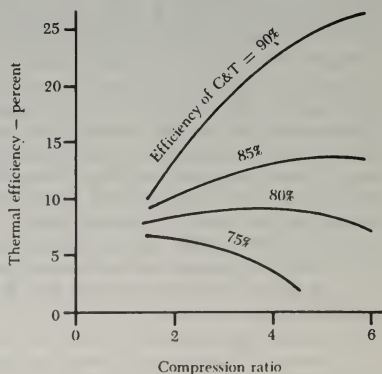
FIGURE 1-72. Turbine and compressor efficiency vs. thermal efficiency.
